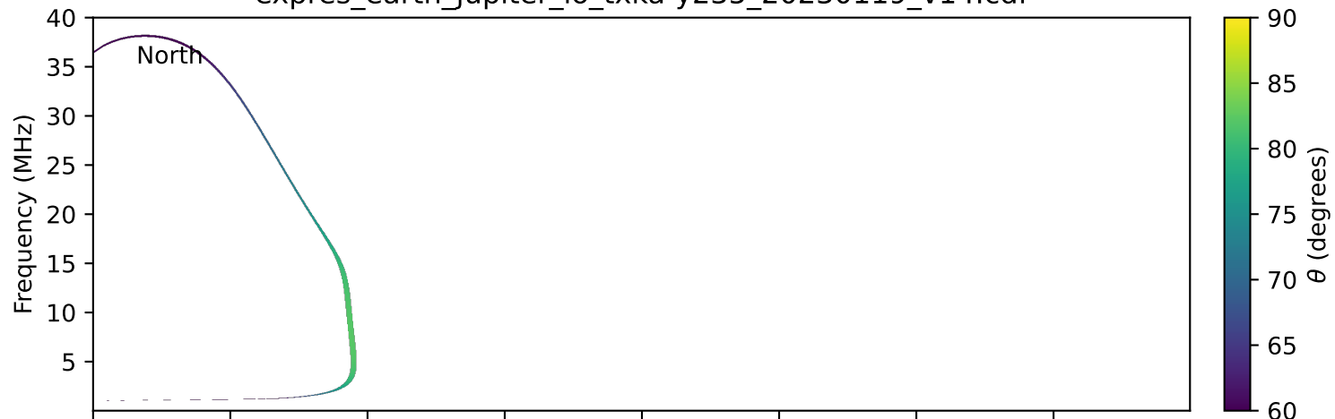
expres_earth_jupiter_io_txka-y235_20230119_v14.cdf
