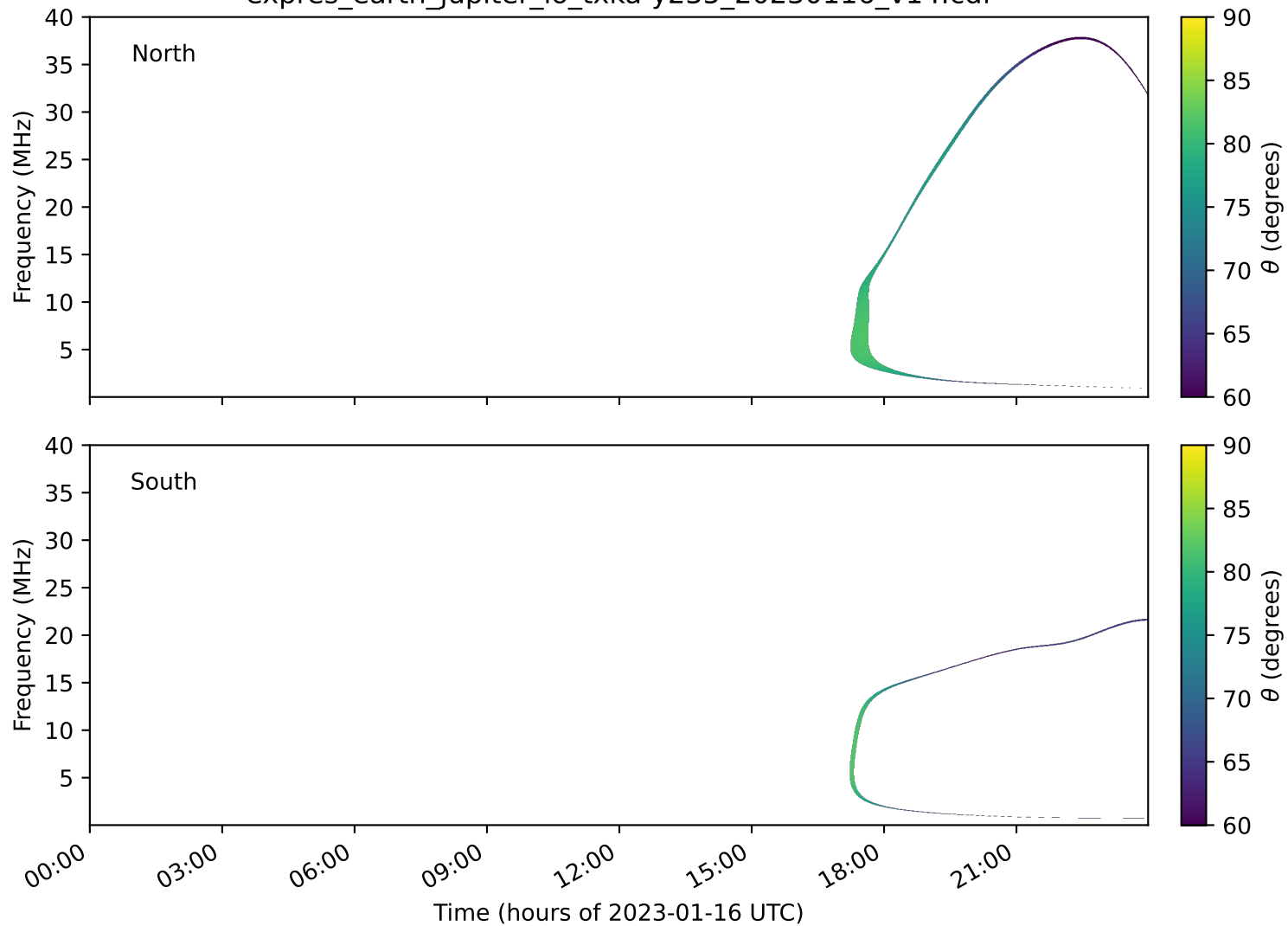
expres_earth_jupiter_io_txka-y235_20230116_v14.cdf
