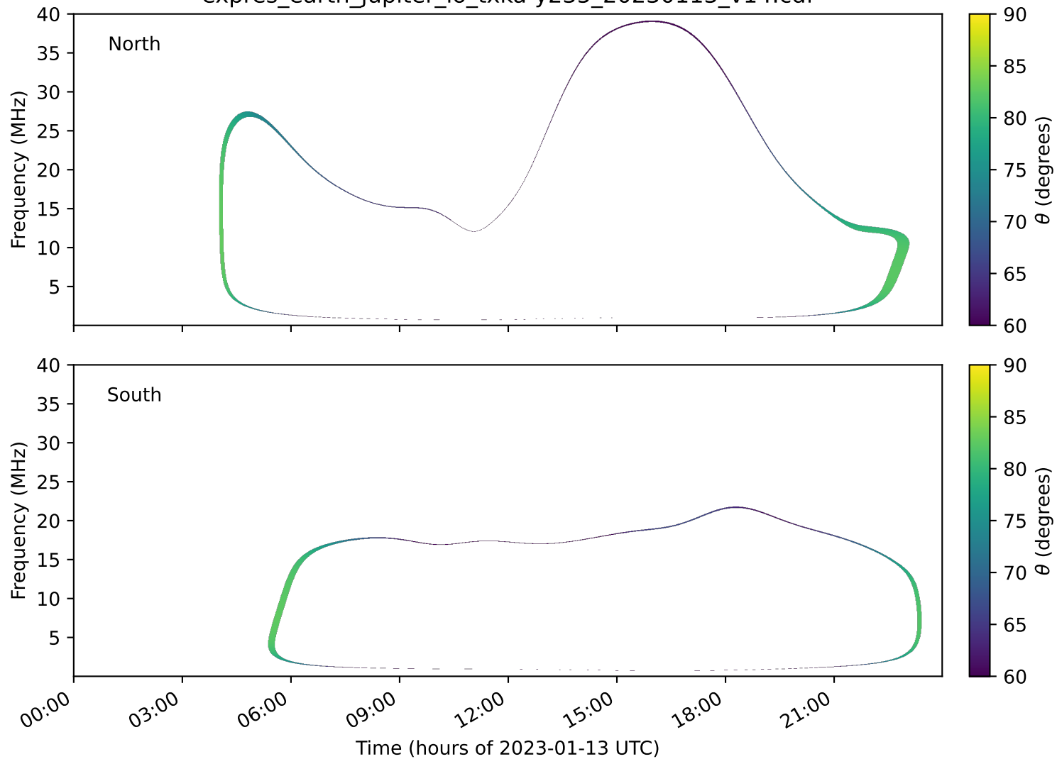
expres_earth_jupiter_io_txka-y235_20230113_v14.cdf
