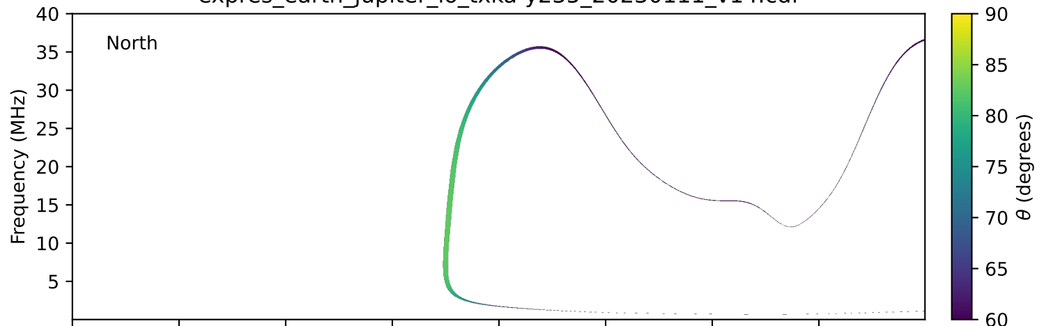
expres_earth_jupiter_io_txka-y235_20230111_v14.cdf
