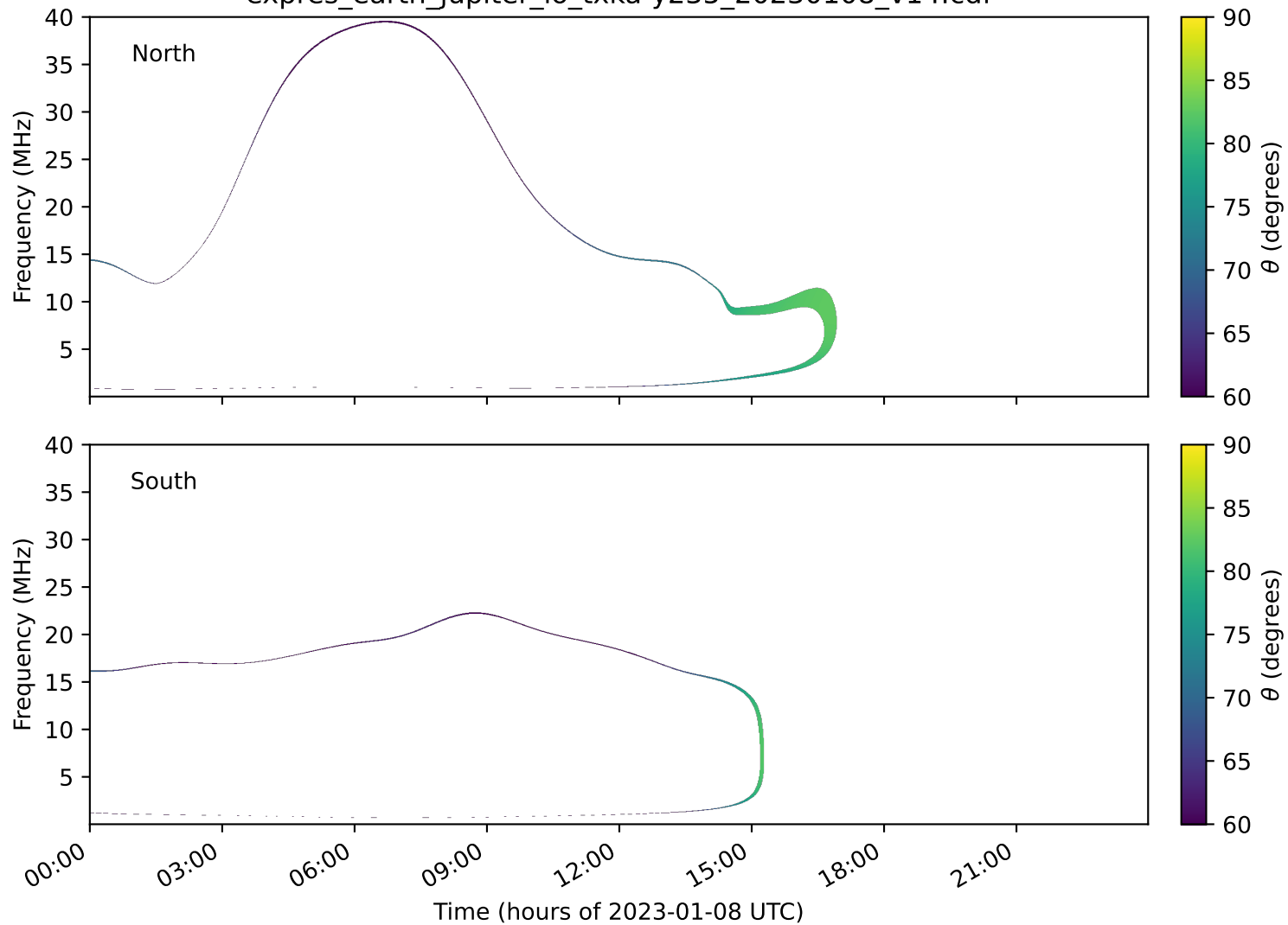
expres_earth_jupiter_io_txka-y235_20230108_v14.cdf
