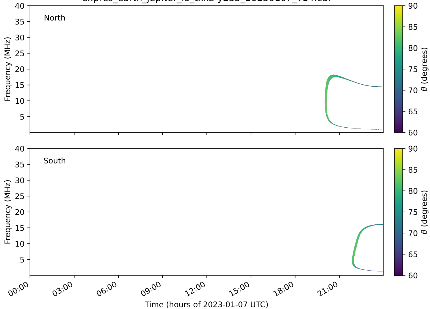
expres_earth_jupiter_io_txka-y235_20230107_v14.cdf
