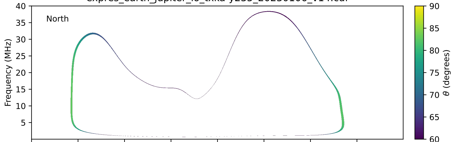
expres_earth_jupiter_io_txka-y235_20230106_v14.cdf
