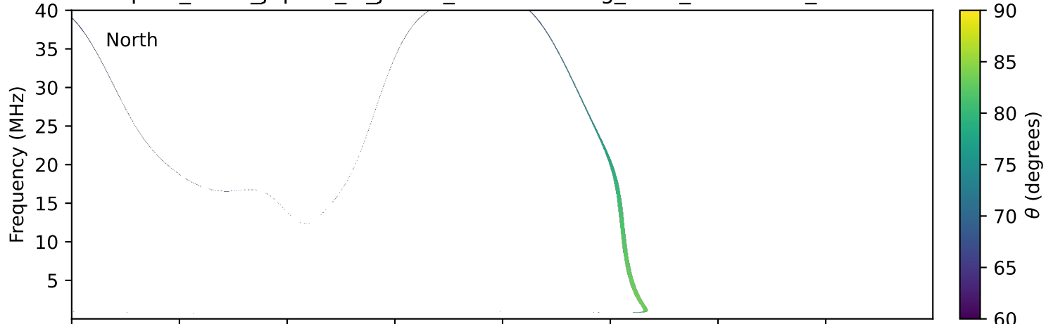
expres_earth_jupiter_io_jrm33_lossc-wid1deg_3kev_20230131_v11.cdf
