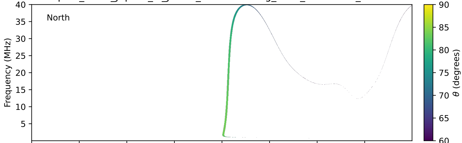
expres_earth_jupiter_io_jrm33_lossc-wid1deg_3kev_20230118_v11.cdf
