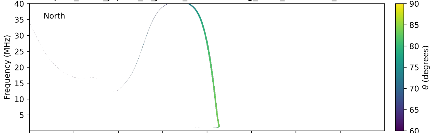
expres_earth_jupiter_io_jrm33_lossc-wid1deg_3kev_20230117_v11.cdf
