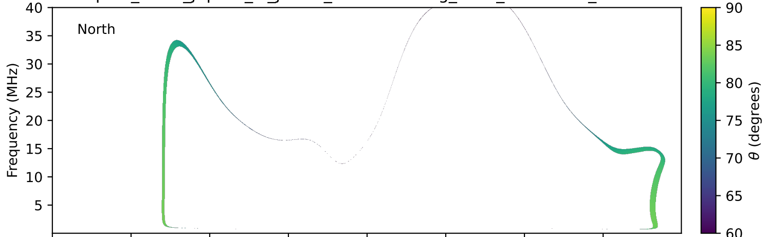
expres_earth_jupiter_io_jrm33_lossc-wid1deg_3kev_20230113_v11.cdf
