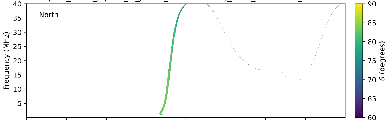
expres_earth_jupiter_io_jrm33_lossc-wid1deg_3kev_20230111_v11.cdf
