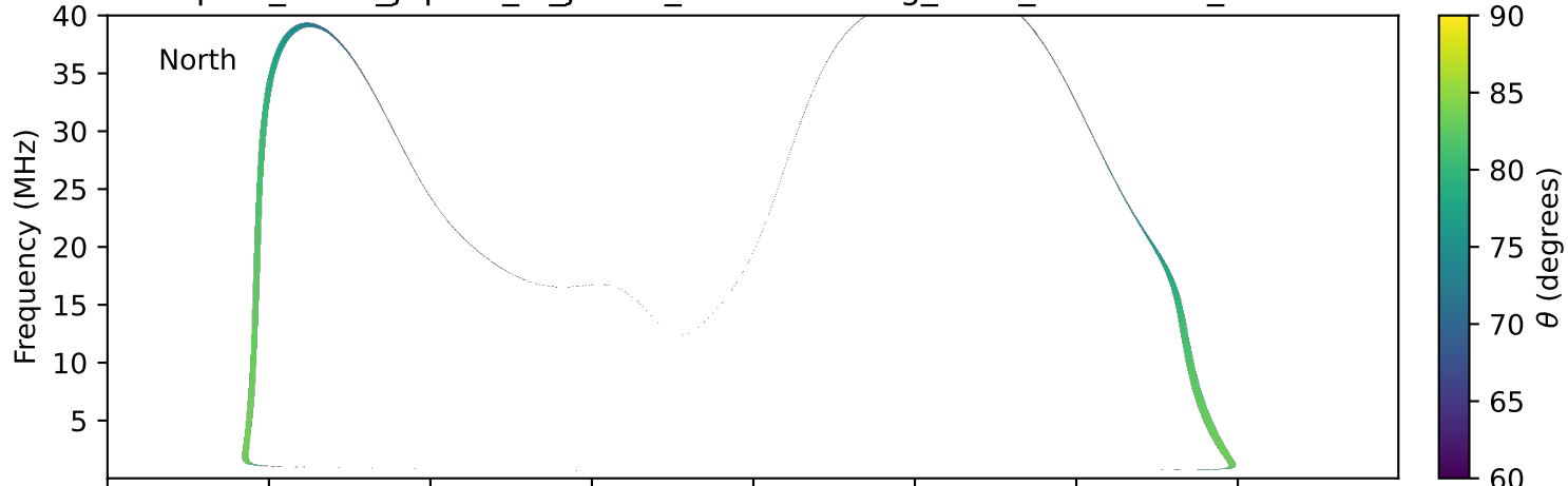
expres_earth_jupiter_io_jrm33_lossc-wid1deg_3kev_20230106_v11.cdf
