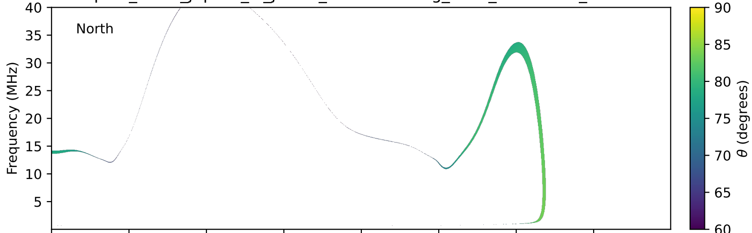
expres_earth_jupiter_io_jrm09_lossc-wid1deg_3kev_20230115_v11.cdf
