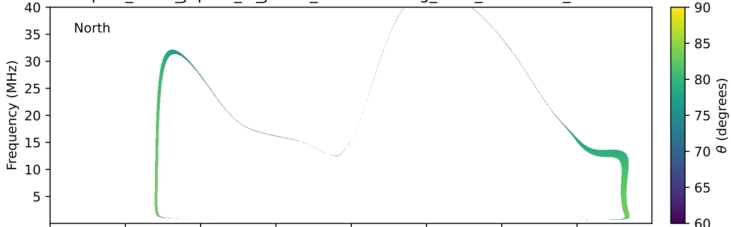
expres_earth_jupiter_io_jrm09_lossc-wid1deg_3kev_20230113_v11.cdf
