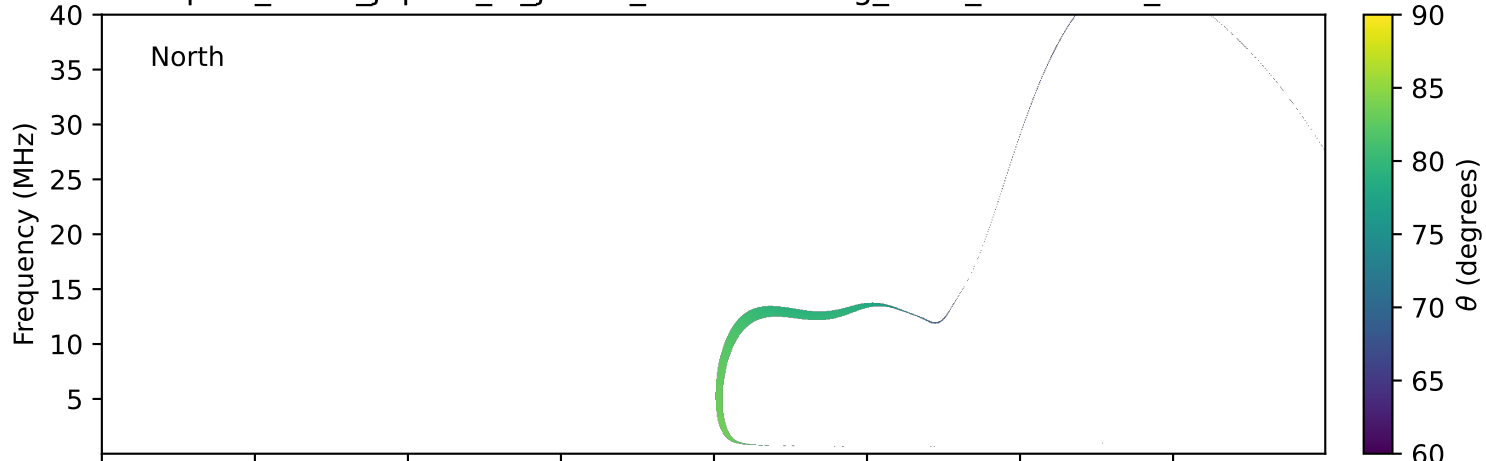
expres_earth_jupiter_io_jrm09_lossc-wid1deg_3kev_20230102_v11.cdf
