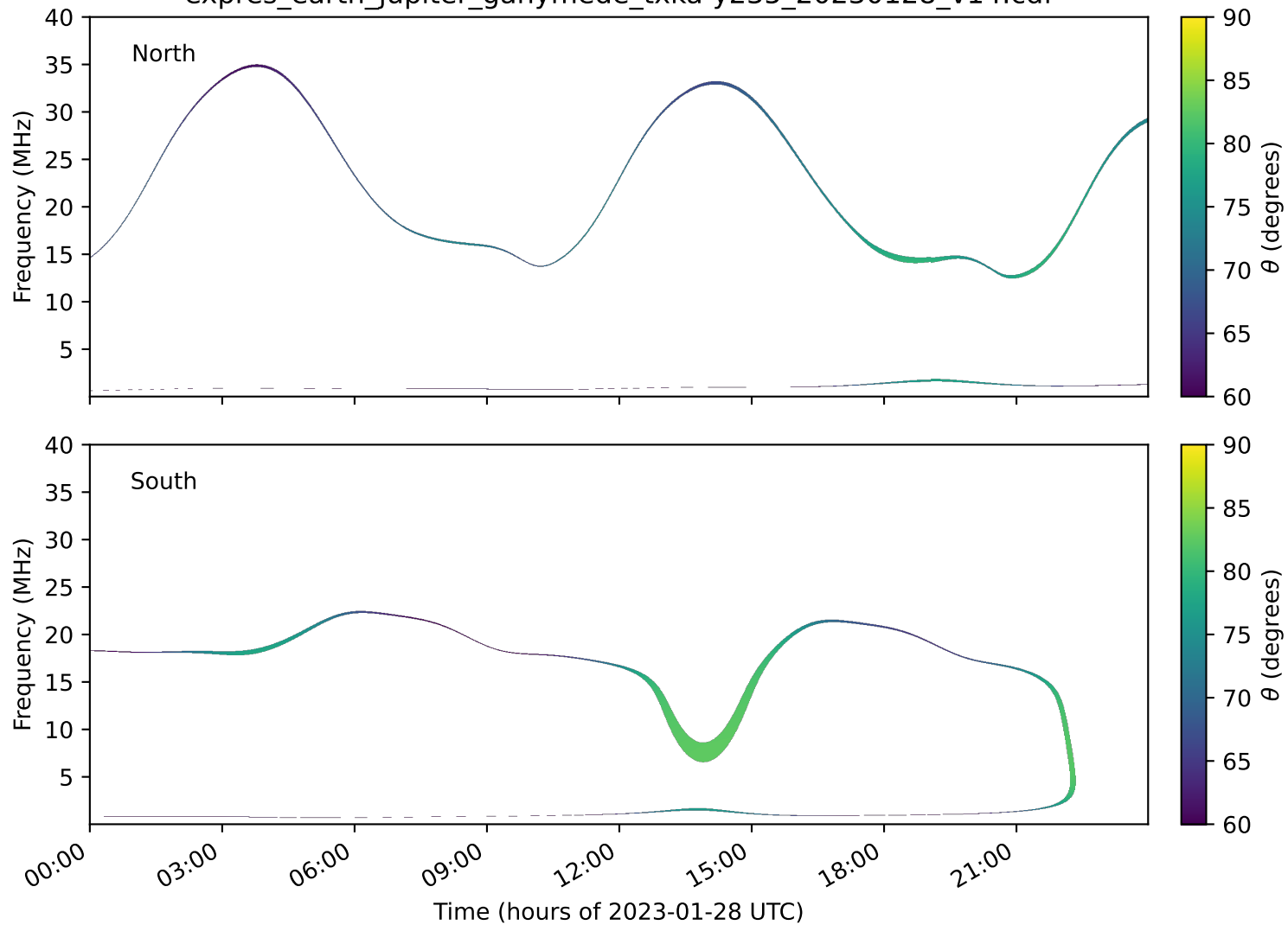
expres_earth_jupiter_ganymede_txka-y235_20230128_v14.cdf
