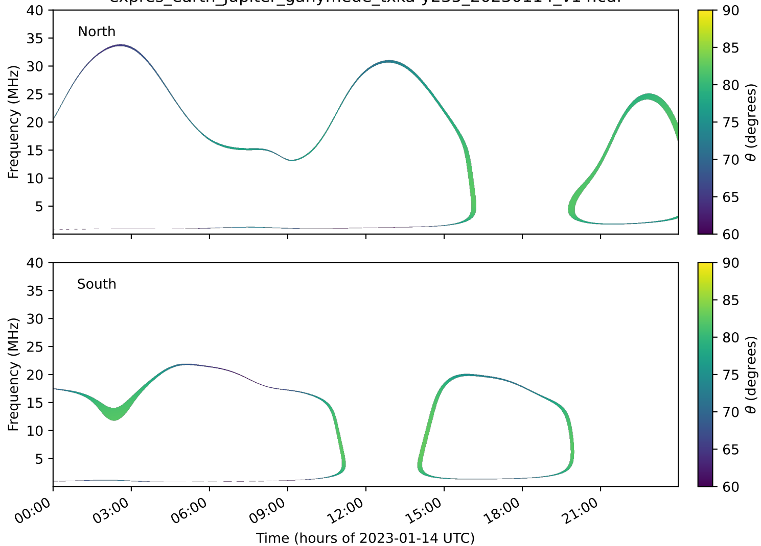
expres_earth_jupiter_ganymede_txka-y235_20230114_v14.cdf
