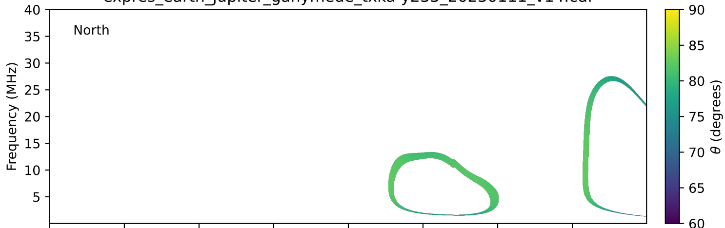
expres_earth_jupiter_ganymede_txka-y235_20230111_v14.cdf
