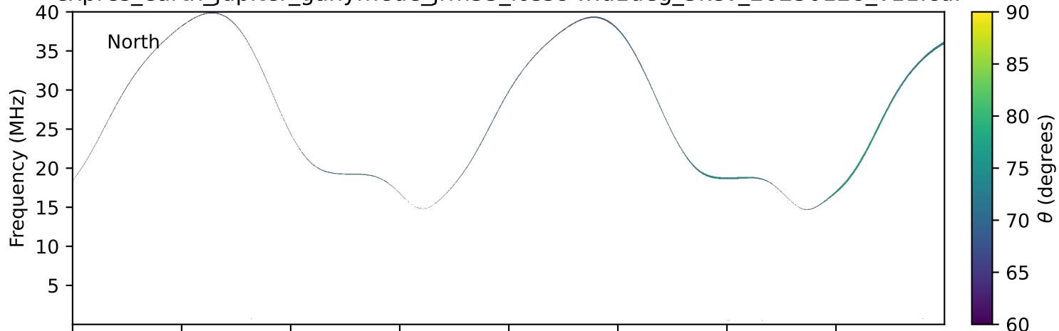
expres_earth_jupiter_ganymede_jrm33_lossc-wid1deg_3kev_20230128_v11.cdf
