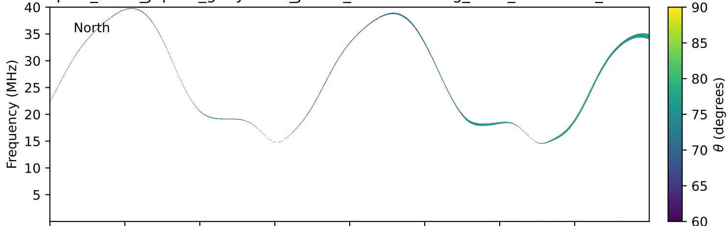
expres_earth_jupiter_ganymede_jrm33_lossc-wid1deg_3kev_20230121_v11.cdf
