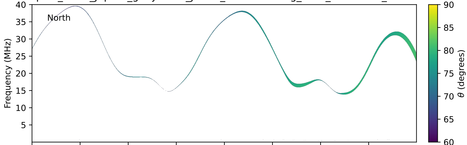
expres_earth_jupiter_ganymede_jrm33_lossc-wid1deg_3kev_20230114_v11.cdf
