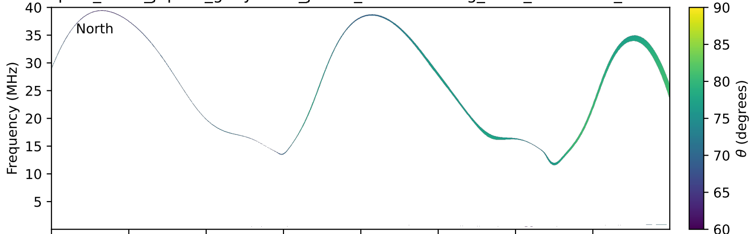
expres_earth_jupiter_ganymede_jrm09_lossc-wid1deg_3kev_20230114_v11.cdf
