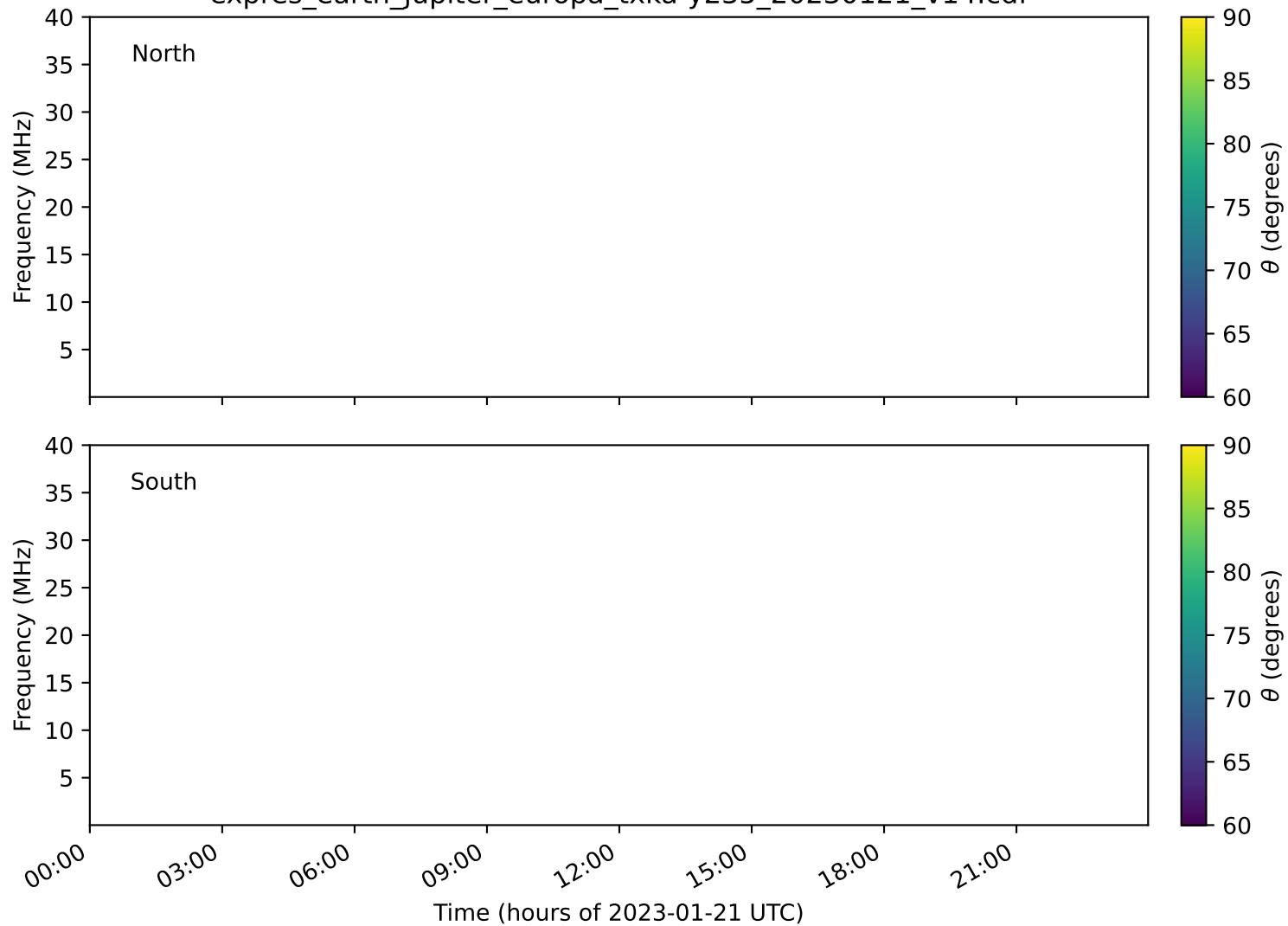
expres_earth_jupiter_europa_txka-y235_20230121_v14.cdf
