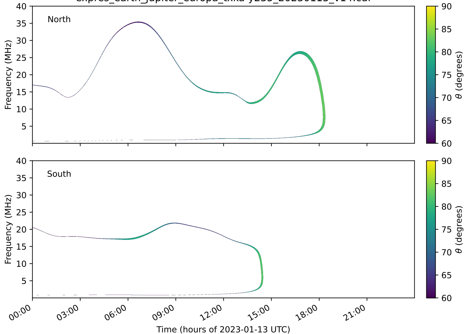
expres_earth_jupiter_europa_txka-y235_20230113_v14.cdf
