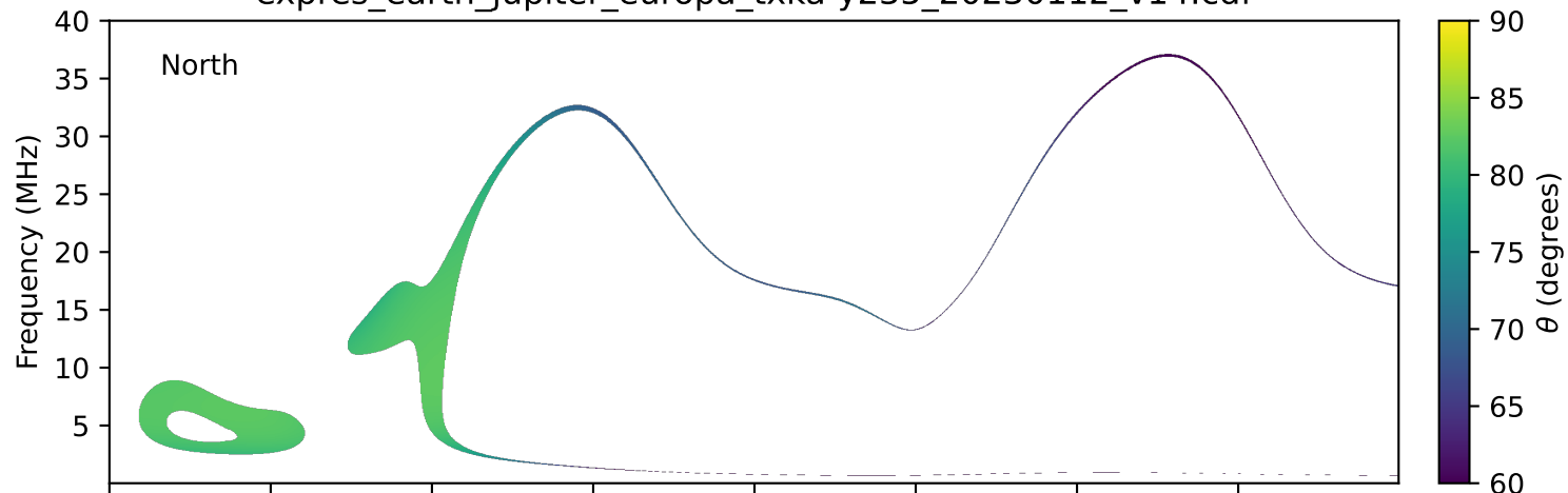
expres_earth_jupiter_europa_txka-y235_20230112_v14.cdf
