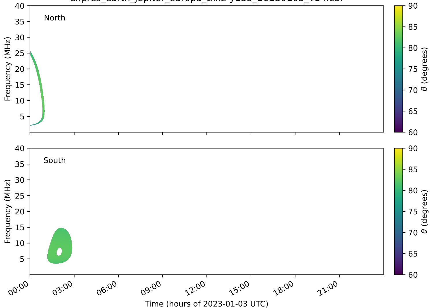
expres_earth_jupiter_europa_txka-y235_20230103_v14.cdf
