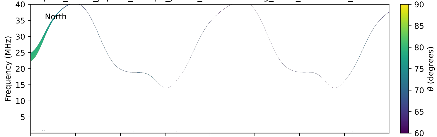
expres_earth_jupiter_europa_jrm33_lossc-wid1deg_3kev_20230123_v11.cdf
