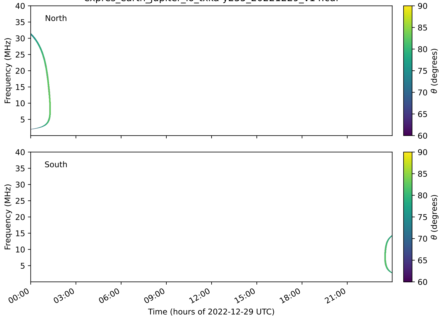
expres_earth_jupiter_io_txka-y235_20221229_v14.cdf
