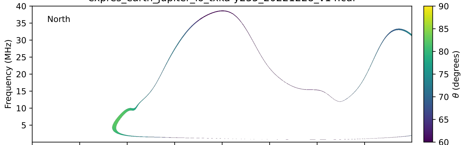
expres_earth_jupiter_io_txka-y235_20221228_v14.cdf
