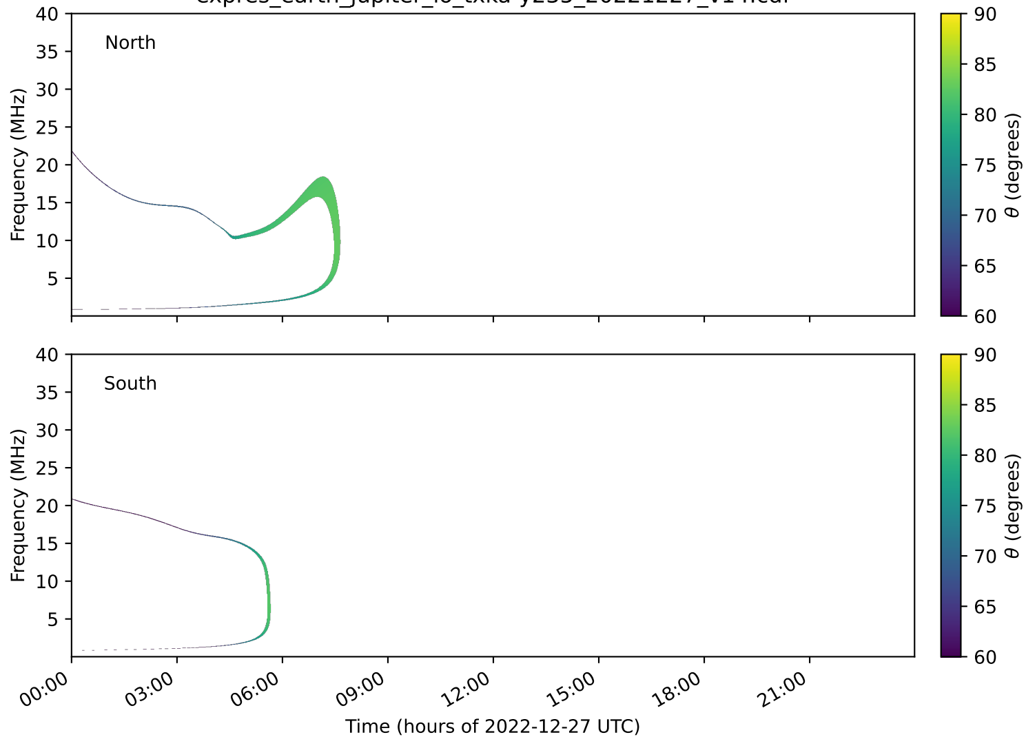
expres_earth_jupiter_io_txka-y235_20221227_v14.cdf
