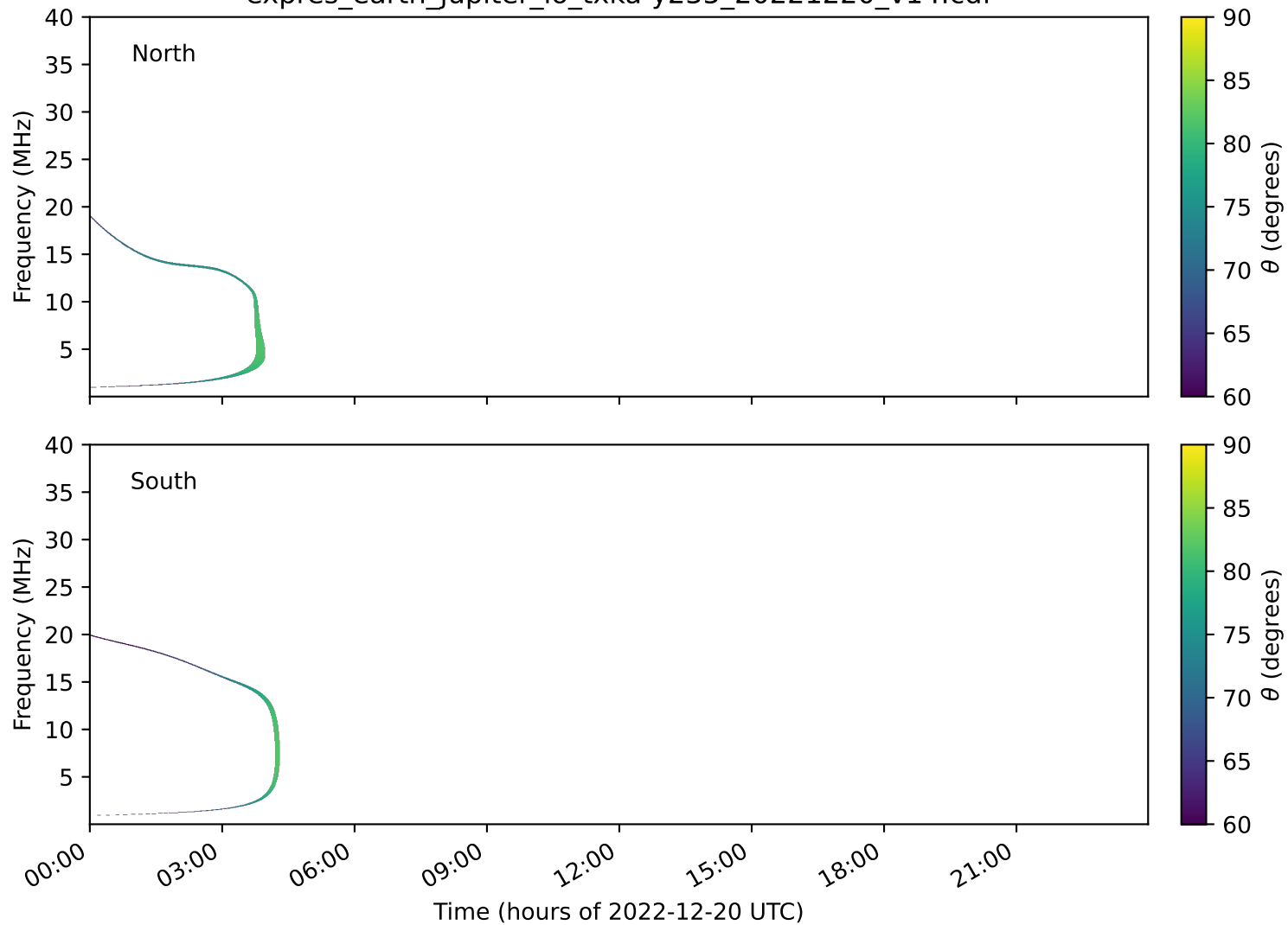
expres_earth_jupiter_io_txka-y235_20221220_v14.cdf
