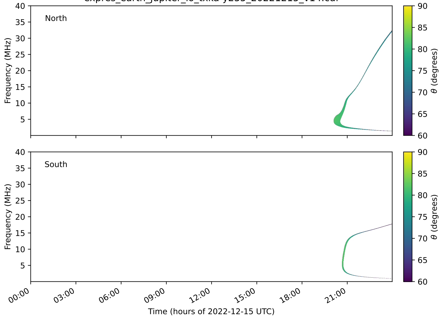
expres_earth_jupiter_io_txka-y235_20221215_v14.cdf
