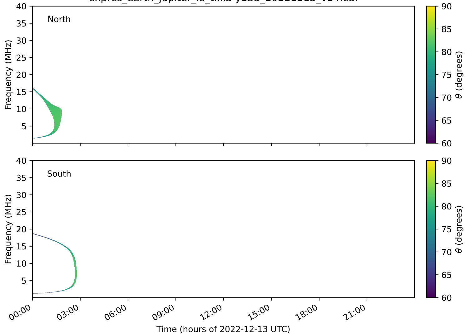
expres_earth_jupiter_io_txka-y235_20221213_v14.cdf
