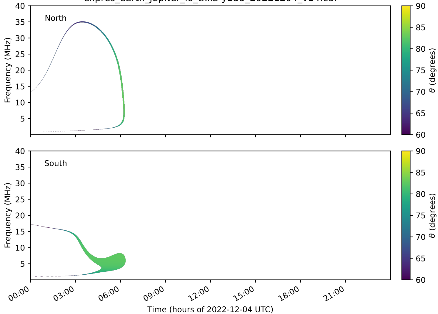
expres_earth_jupiter_io_txka-y235_20221204_v14.cdf
