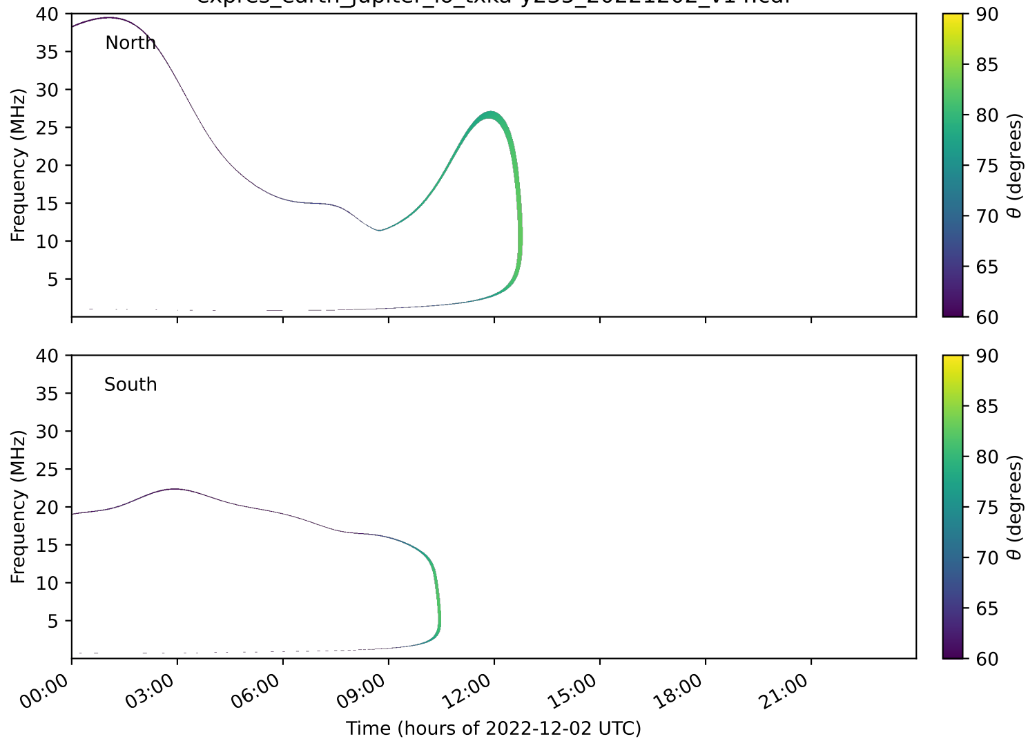
expres_earth_jupiter_io_txka-y235_20221202_v14.cdf
