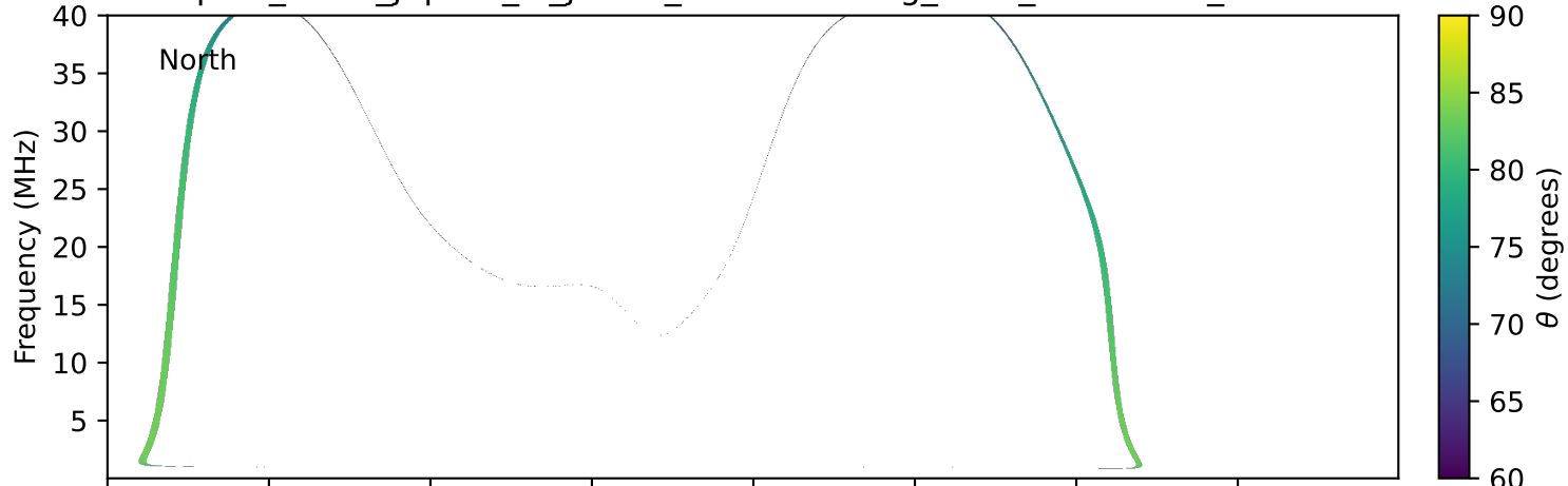
expres_earth_jupiter_io_jrm33_lossc-wid1deg_3kev_20221230_v11.cdf
