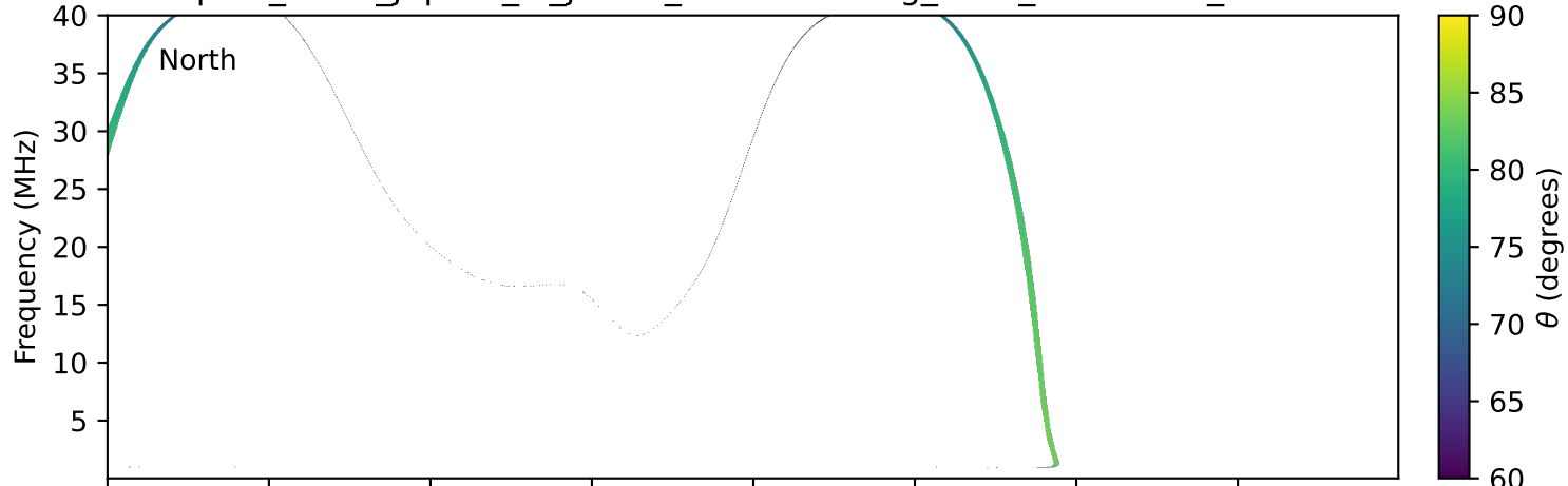
expres_earth_jupiter_io_jrm33_lossc-wid1deg_3kev_20221223_v11.cdf
