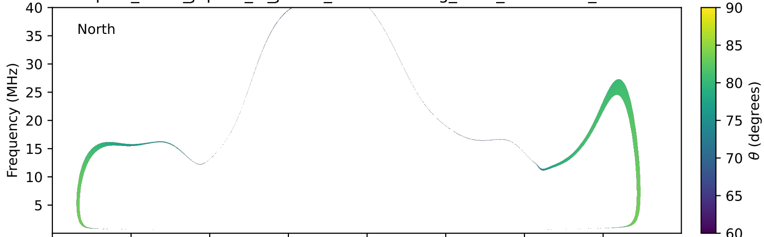
expres_earth_jupiter_io_jrm33_lossc-wid1deg_3kev_20221214_v11.cdf
