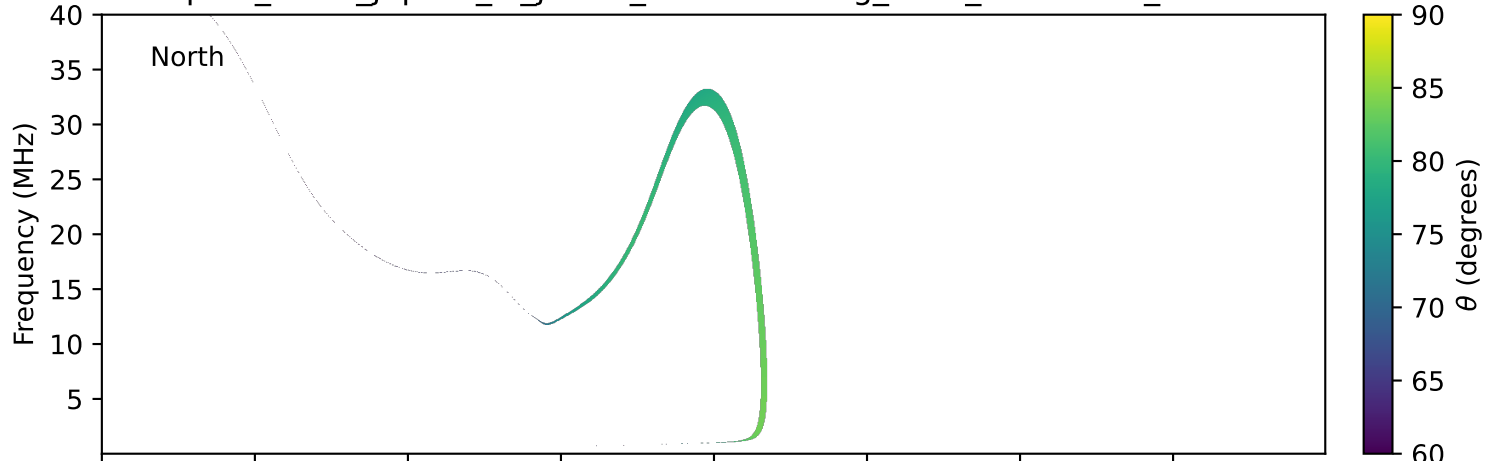
expres_earth_jupiter_io_jrm33_lossc-wid1deg_3kev_20221202_v11.cdf
