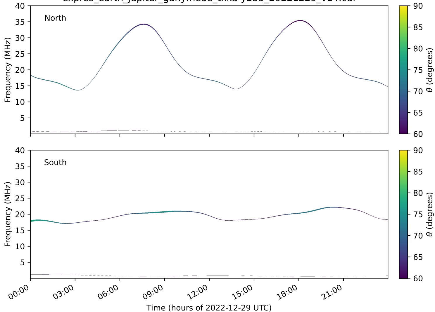
expres_earth_jupiter_ganymede_txka-y235_20221229_v14.cdf
