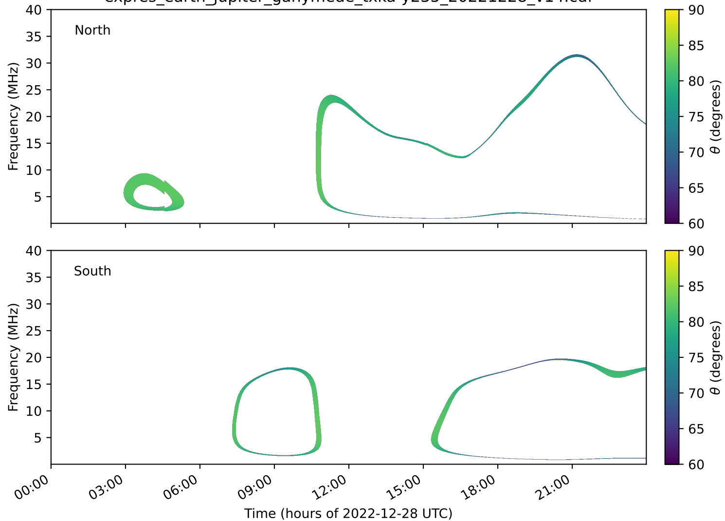
expres_earth_jupiter_ganymede_txka-y235_20221228_v14.cdf
