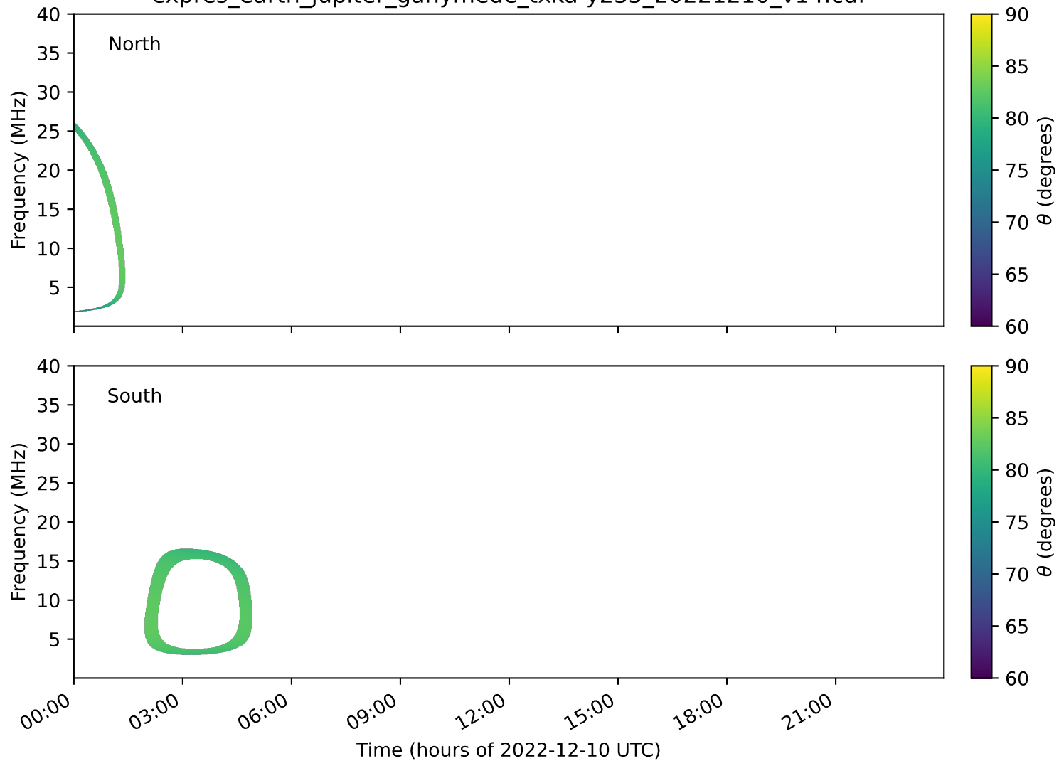
expres_earth_jupiter_ganymede_txka-y235_20221210_v14.cdf
