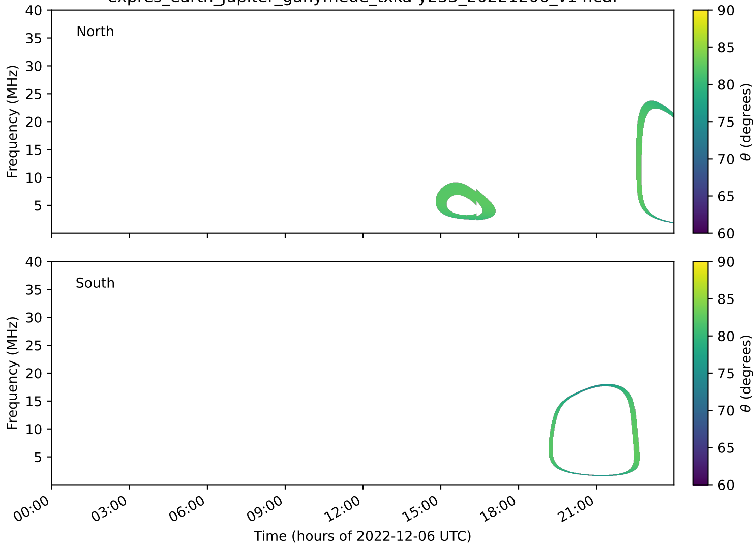
expres_earth_jupiter_ganymede_txka-y235_20221206_v14.cdf
