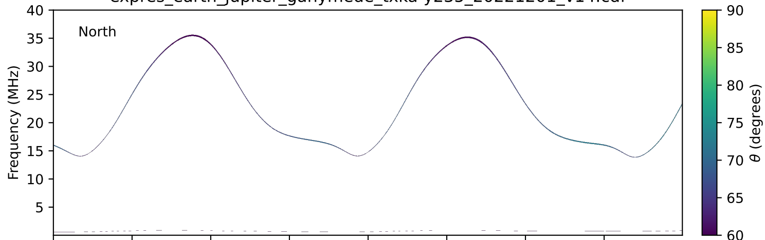
expres_earth_jupiter_ganymede_txka-y235_20221201_v14.cdf
