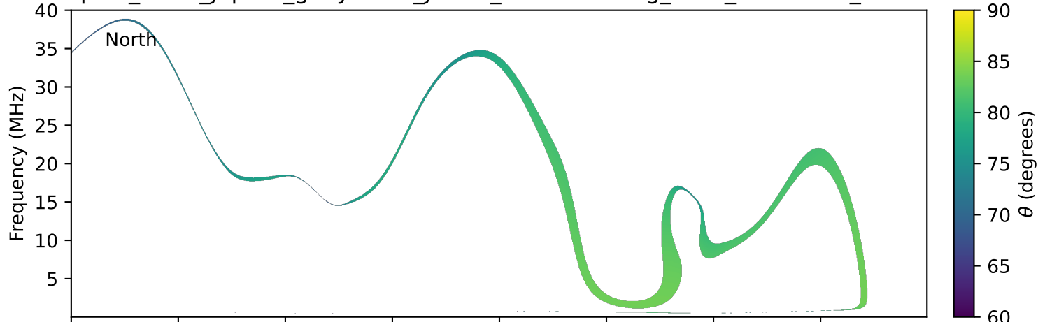
expres_earth_jupiter_ganymede_jrm33_lossc-wid1deg_3kev_20221231_v11.cdf
