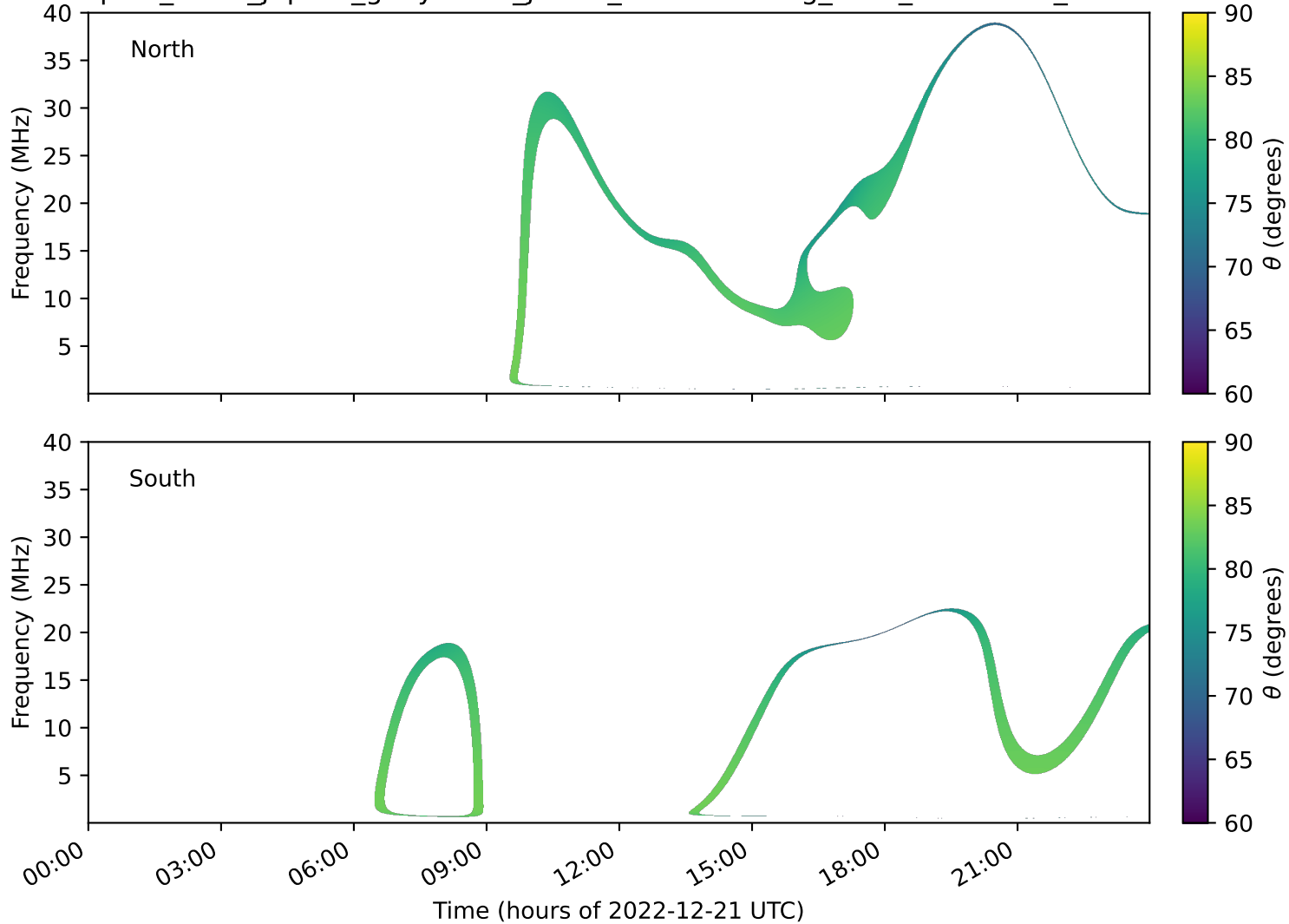
expres_earth_jupiter_ganymede_jrm33_lossc-wid1deg_3kev_20221221_v11.cdf
