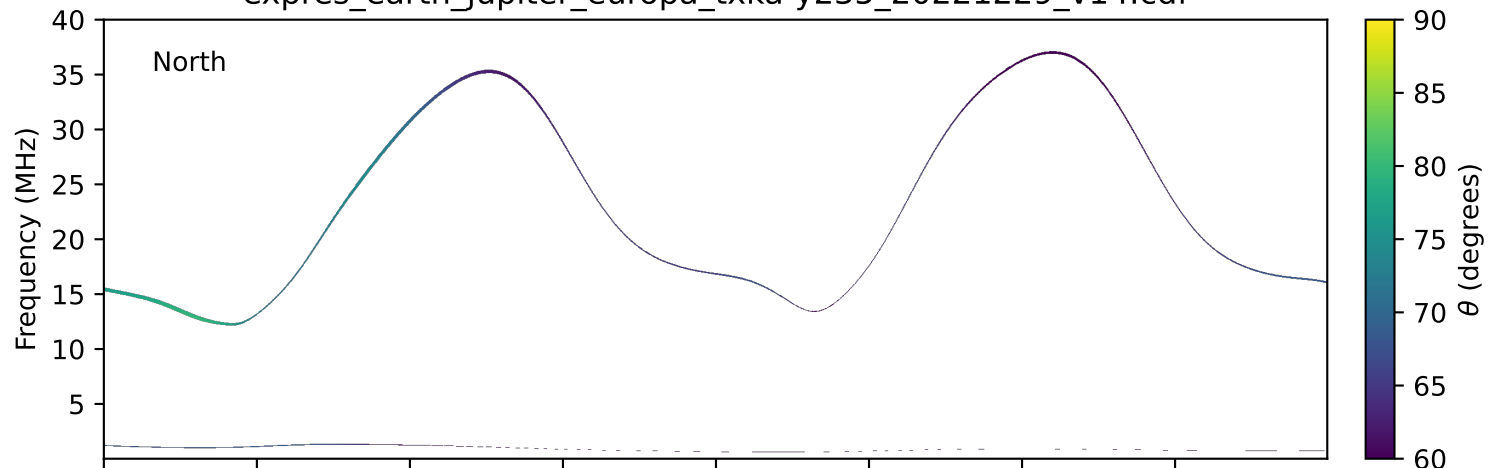
expres_earth_jupiter_europa_txka-y235_20221229_v14.cdf
