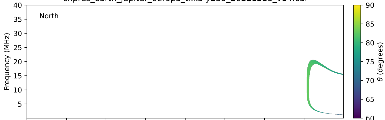
expres_earth_jupiter_europa_txka-y235_20221228_v14.cdf
