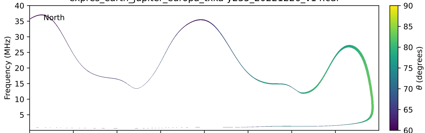
expres_earth_jupiter_europa_txka-y235_20221226_v14.cdf
